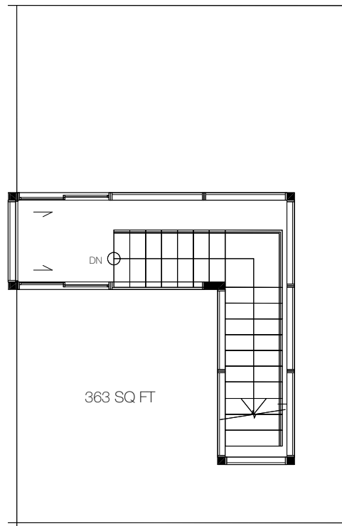
LEVEL 18
